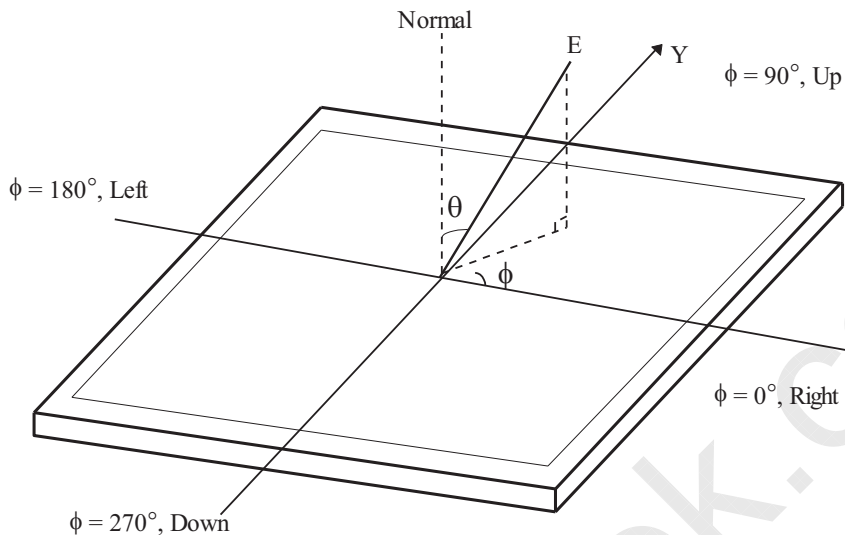
FIG. 10 Viewing angle
