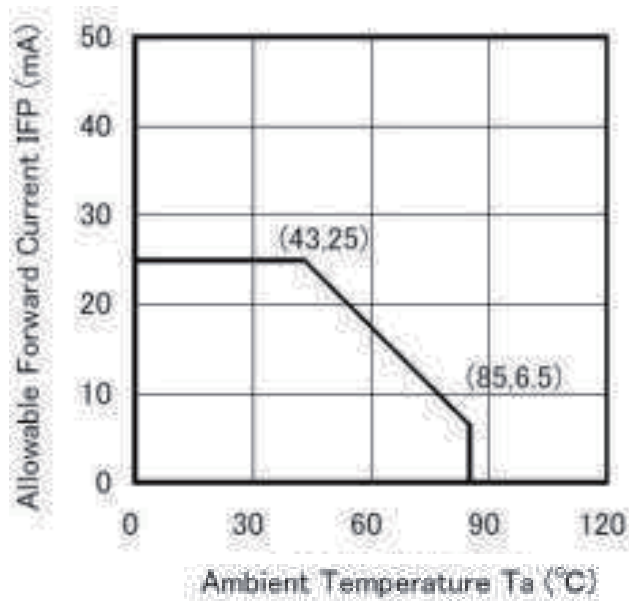
Fig 2.1 Ambient Temperature vs. Allowable Forward Current
